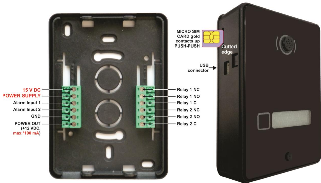
Figure 1: SOLO-IDEA Connection diagram
